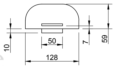
View B-B
