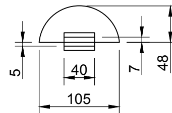
View B-B
