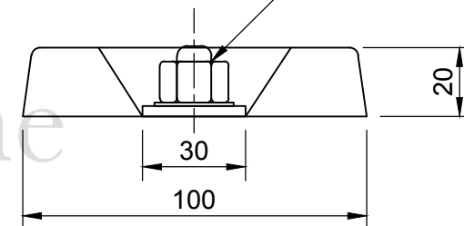
Section B-B Bolt and nut M12x20L
